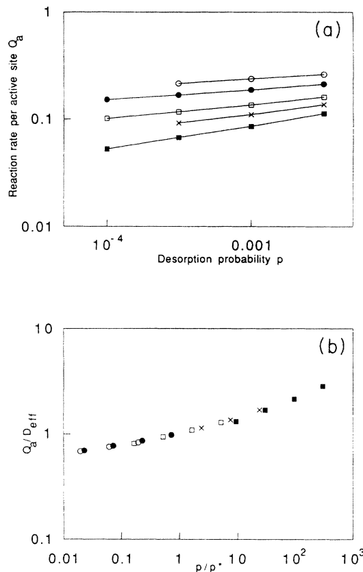
FIG. 6. Reaction rate Q_a for a poisoned 2D lattice at concentrations higher than c_0 : empty circles, c = 0.95 ; solid circles, c = 0.85 ; empty squares, c = 0.75 , Xc = 0.70 ; solid squares, c = 0.65 . (a) Reaction rate versus desorption probability. Full lines are guides to the eyes. (b) Scaled reaction rate versus scaled desorption probability.
